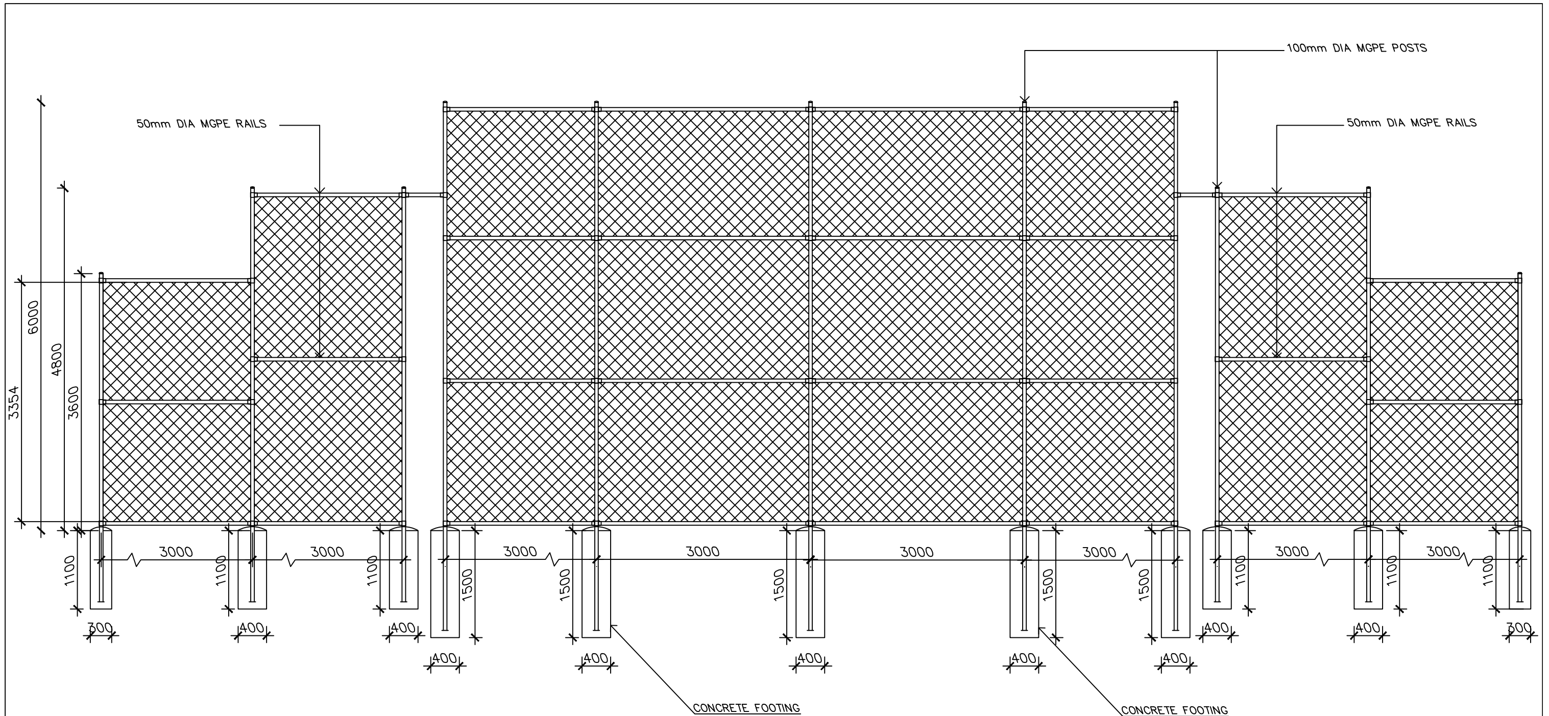
1 ELEVATION — NTS
